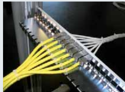
Alien Crosstalk arrangement by using MegaLineNet®: 6 "disturber" and 1 "victim"
